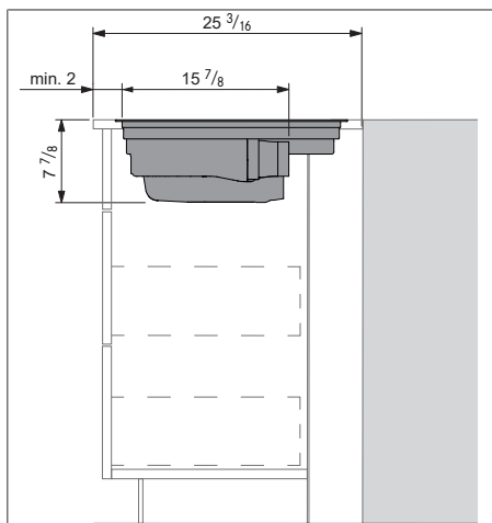
Fig. 11.15 Installation dimensions for exhaust air, worktop depth 25 \frac{3}{16} " [64 cm]
