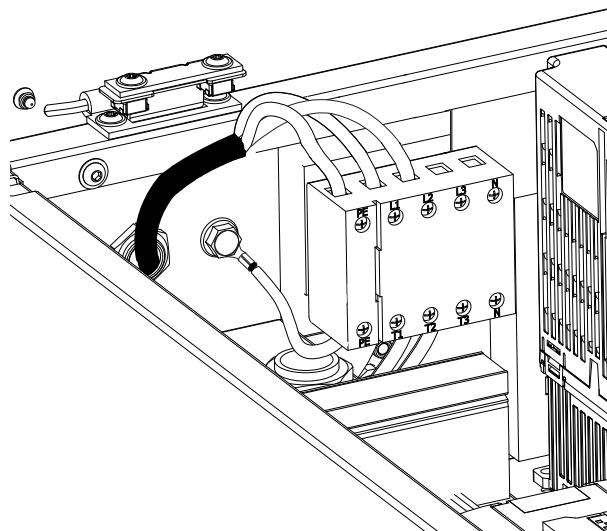
NAR Single Phase Connection (L1-L2)
