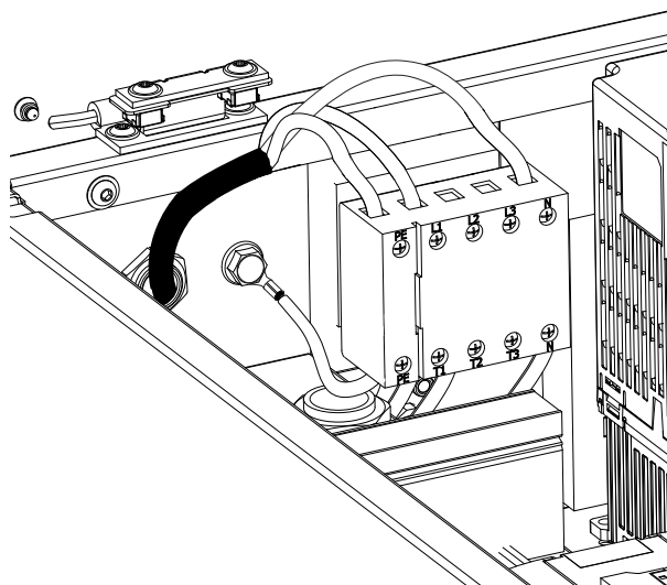
International Single Phase Connection (L1-N)
