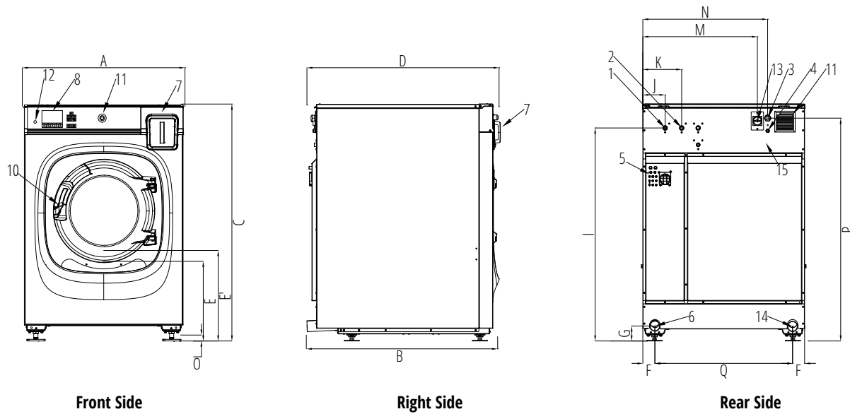
Fig. 1.3 Front, right and rear side view diagrams of MWS85 models
