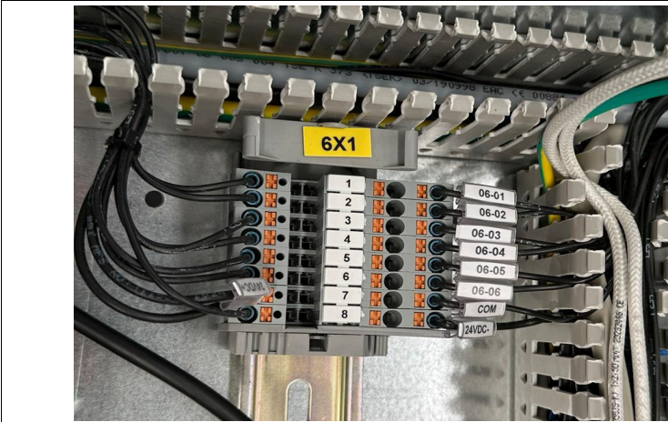
Fig. 4.7 Location and Detail of the 6X1 Detergent Signal Terminal
