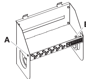
A. Phillips-head screw (F3b) B. Acorn nut (F10)
