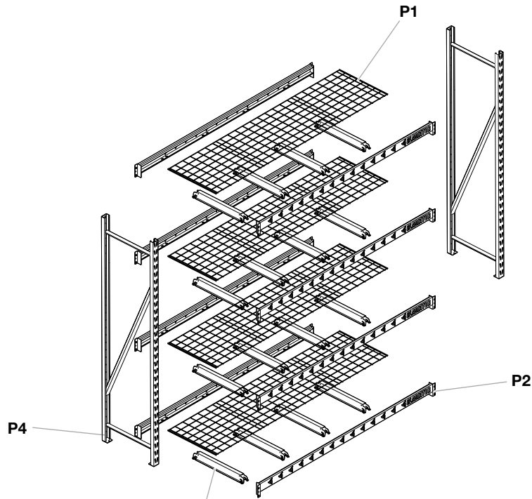
P3 90" (229 cm) Wide Rack Shelving
