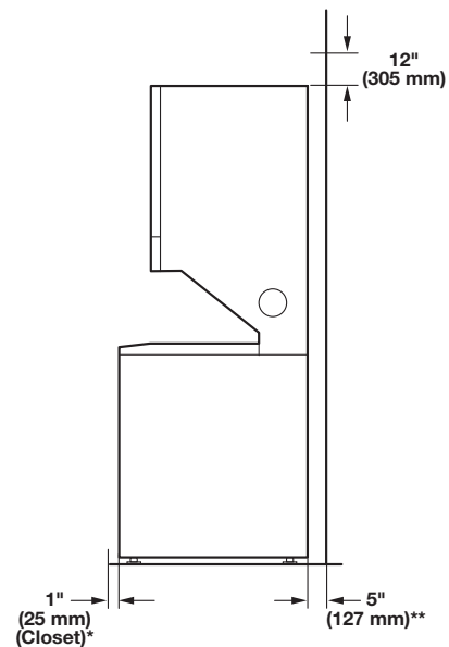
Front/Back/Top Clearances
