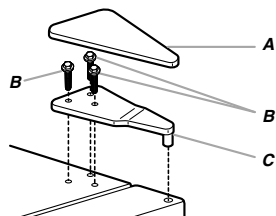
A. Top Hinge Cover B. 5/16" Hex-Head Hinge Screws C. Top Hinge
