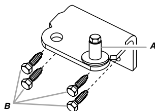
A. Hinge Pin B. 3/8" Hex-Head Hinge Screws
