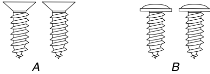
A. #8 x 5/8" Phillips flat-head wood screws B. Phillips color-matched toekick screws
