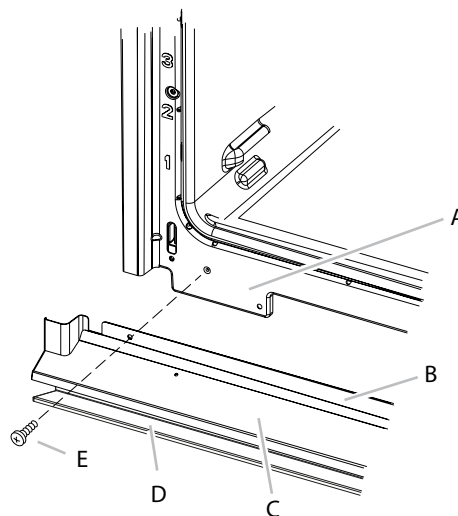
A. Oven frame B. Vent tab C. Oven vent D. Bottom vent trim E. #8-18 x \frac{3}{8} " screws
