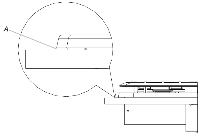
A. Small gap (approximately \frac{1}{8} " [3 mm]) between cooktop and countertop
