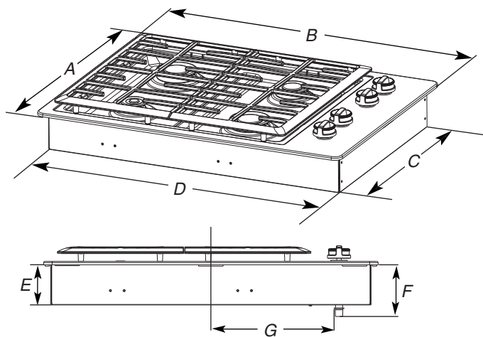
30" (76.2 cm) Model (W5CG3024)
