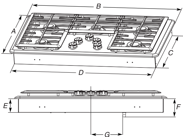
36" (91.4 cm) Model (W5CG3625)
