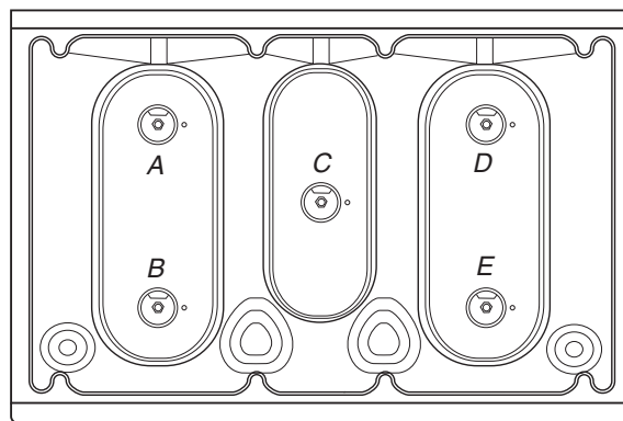
A. Standard burner - Natural gas orifice spud number 125 B. Power burner - Natural gas orifice spud number 132 C. Center burner - Natural gas orifice spud number 128 D. Standard burner - Natural gas orifice spud number 125 E. Standard burner - Natural gas orifice spud number 125
