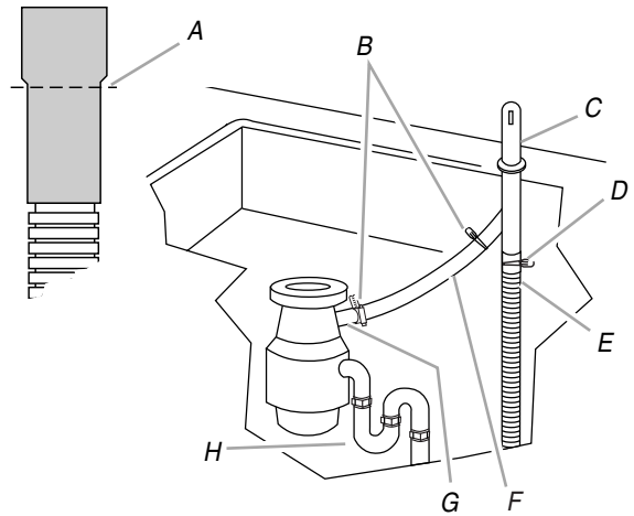
A. Drain hose—cut here, if needed B. Spring- or screw-type clamps C. Air gap D. Large spring-type clamp
