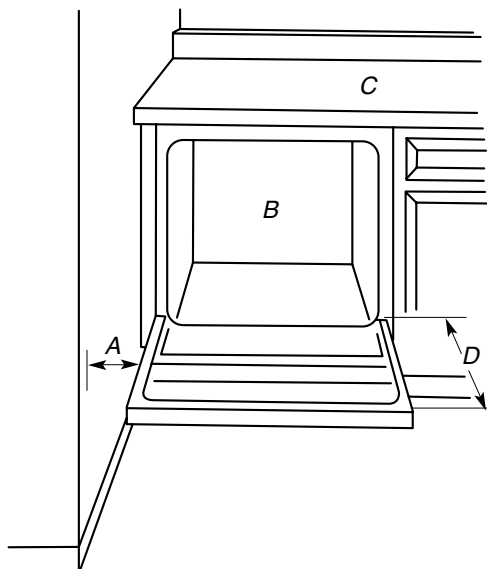
A. 2" (5.1 cm) minimum clearance for door opening B. Dishwasher
