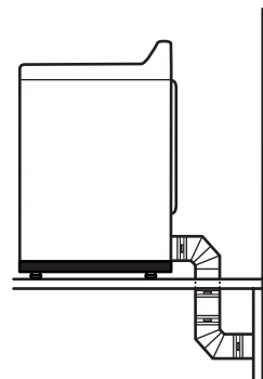
Mobile Home Exhaust installation
