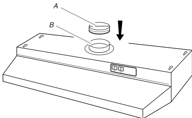
A. 7" (17.8 cm) Round damper (supplied) B. 7" (17.8 cm) Round discharge collar
