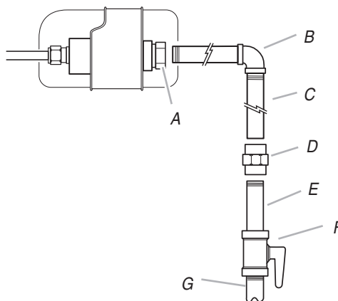
A. Pressure regulator connection fitting B. 90° elbow C. Black iron pipe
