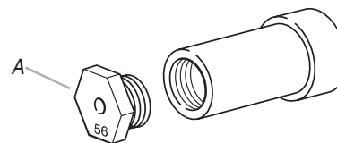
A. LP oven orifice spud stamped with "56"
