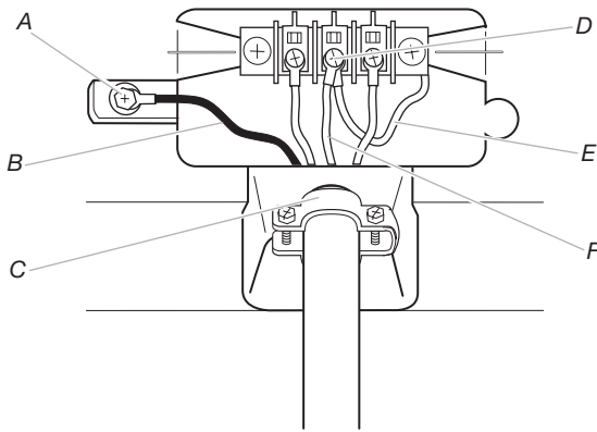
A. External ground conductor screw B. Ground wire (green or bare) of power supply cord C. \frac{3}{4} " (19 mm) UL listed strain relief D. Center, silver-colored terminal block screw E. Neutral ground wire F. Neutral wire (white or center wire)
