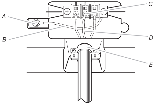
A. External ground conductor screw B. Neutral ground wire C. Center silver-colored terminal block screw D. Neutral wire (white or center wire) E. 3/4" (19 mm) UL listed strain relief
