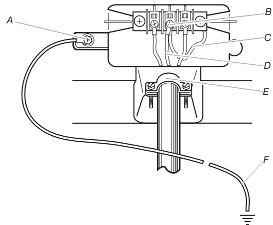
A. External ground conductor screw B. Center silver-colored terminal block screw C. Neutral ground wire D. Neutral wire (white or center wire) E. 3/4" (19 mm) UL listed strain relief F. Grounding path determined by a qualified electrician
