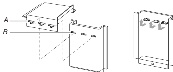
A. Tabs of upper duct
