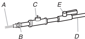
A. ¾" flexible gas connector B. ¾" pipe to flare adapter fitting C. ⅛" NPT plugged tapping D. ½" NPT gas supply line E. Gas shutoff valve
