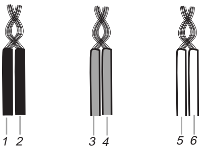
1. Black wire 2. Incoming L1 wire (black wire) 3. Green wire 4. Ground wire (green wire) 5. White wire 6. Neutral wire (white wire)
